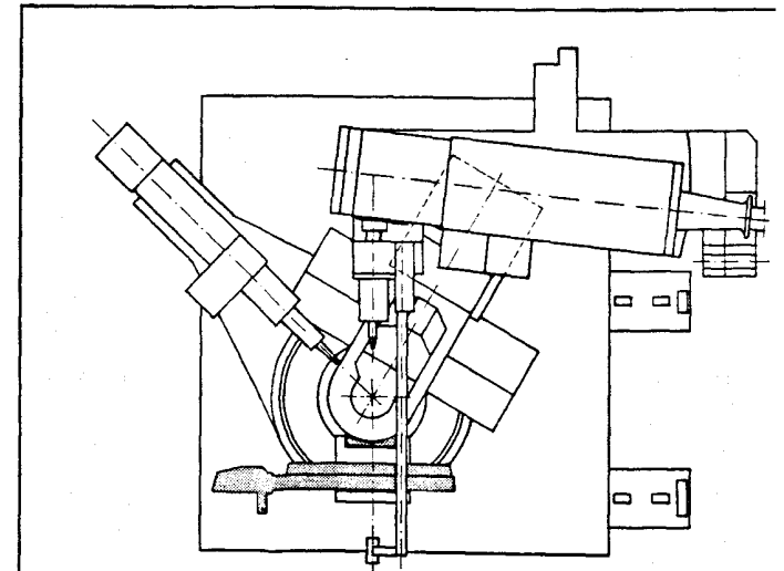
FIG. 20 STANDARD POLAROID CASSETTE BRACKET FITTED TO CAD4 GONIOMETER. FOR DETAILS SEE FIG. 12
